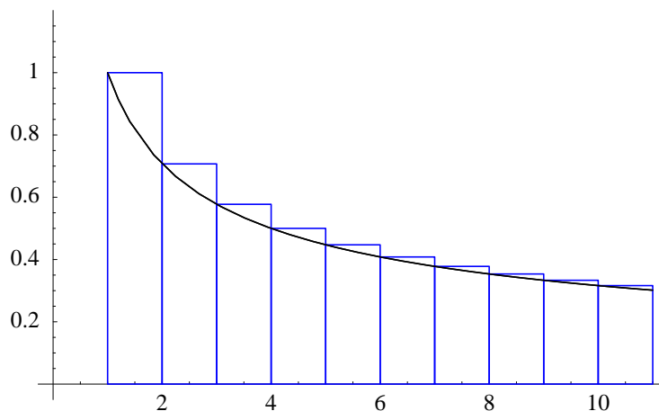
Figure 5.3.1 Rectangles for left-hand rule approximation for \int_1^{11} \frac{1}{\sqrt{x}} dx
