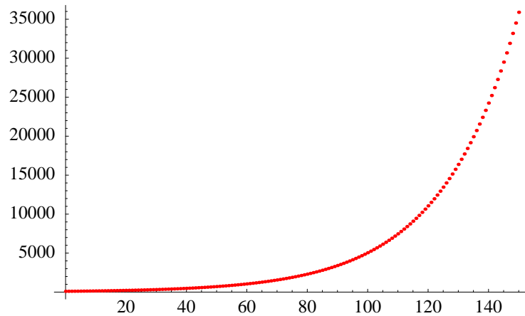
Figure 1.5.2 Uninhibited population growth with \beta = 0.04
